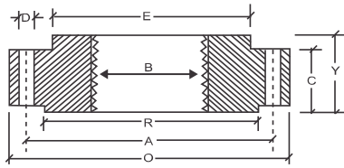
THREADED FLANGES
