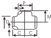
REDUCING TEES
