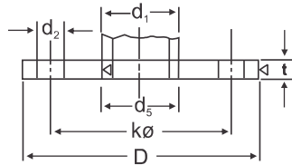
SLIP-ON
