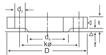
BLIND
