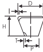
CONCENTRIC REDUCERS
