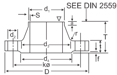
WELDING NECK
